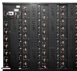
20KWh LifePO4
