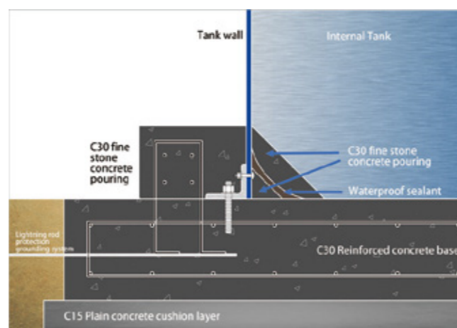
Above-Floor Foundation
