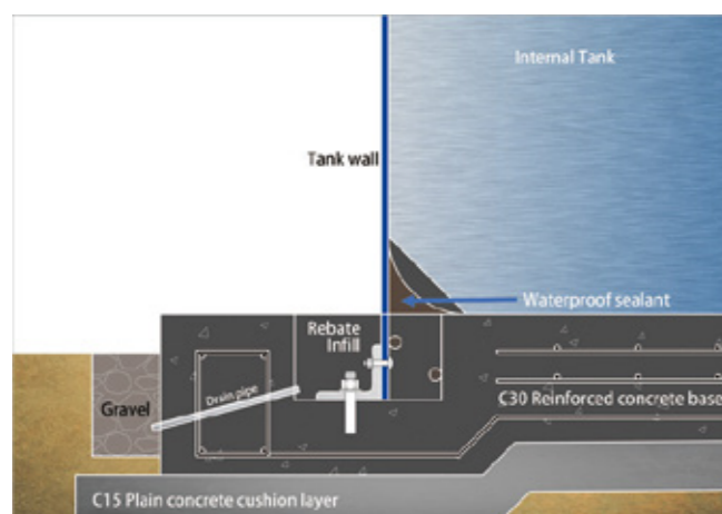
Embedded Foundation
